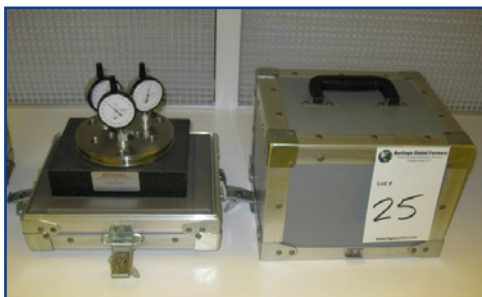
Neutronix Wafer Surface Measurement Device
