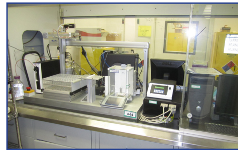
Waters Liquid Handling System: Includes (1) Waters 2767 sample manager (1) Waters TCM (1) Waters heat module (1) Waters 600 Controller (1) Waters In-Line Degasser AF (1) 2487 Dual Absorbance Detector (1) Edwards 28 Pump (1) Dell Computer and monitor
