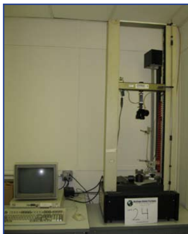
Intech 2 Elastomeric Tester
