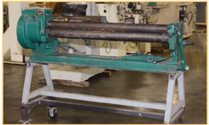
TENNSMITH 48" X 16-GA. MECHANICAL PLATE BENDING ROLLS
