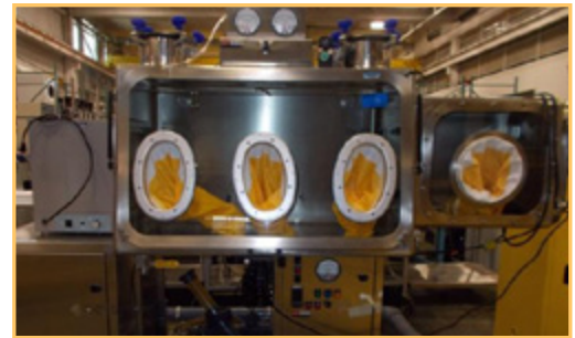
ISOTECH DESIGN ISOPROTECT MOBILE ENVIRONMENTAL CONTROLLED CHAMBER GLOVE BOX
