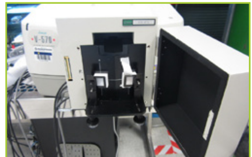
JASCO V-570 UV/VIS AND NIR MEASUREMENT
