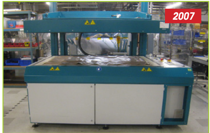
MEIER ICOLAM 18/11 VACUUM LAMINATOR W/ SE-504 CONTROLLER. MFG. 2007
