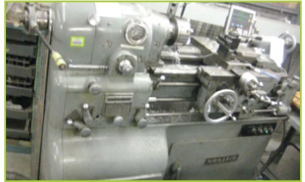
MONARCH EE 10X20 INDUSTRIAL LATHE
