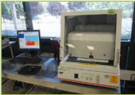
FISCHER XDAL X-RAY SPECTROMETER
