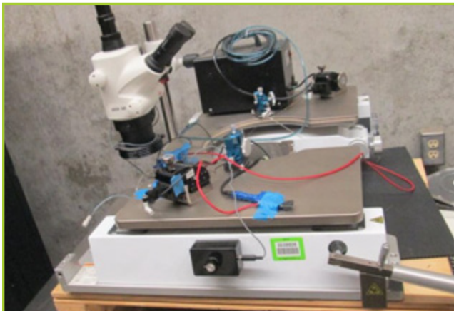
CASCADE MICROTECH M150 150 MM PROBING STATION
