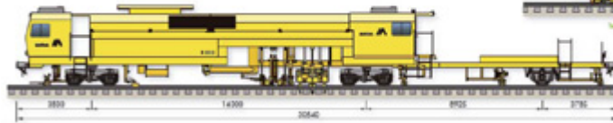
CONTINUOUS ADVANCE LEVELLING AND LINING TAMPER
