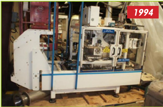
1994 ELMAR RPE-714IHL 14 HEAD ROTARY PISTON FILLER
