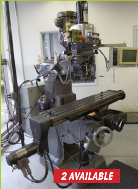
BRIDGEPORT MDL: EZTRAK DX 2 AXIS CNC VERTICAL MILLING MACHINE
