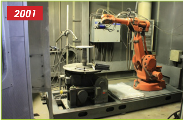
SULZER METCO MULTI COAT AIS PLASMA THERMAL COATING SYSTEM
