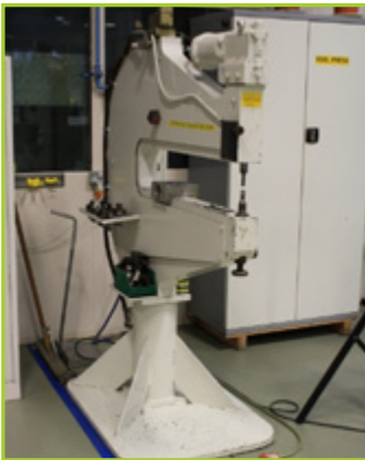
HARDWARE INSERTION/RIVETING PRESS, 36"
