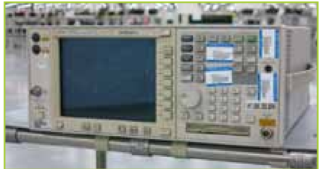
AGILENT E4406A FREQUENCY RANGE RF INPUT: 7 TO 314 MHZ AND 329 MHZ TO 4 GHZ, BASEBAND IQ INPUTS: 0 HZ TO 5 MHZ FREQUENCY SPANS: BASEBAND IQ INPUTS: 5 HZ TO 5 MHZ (BASEBAND I OR Q INPUTS) 10 HZ TO 10 MHZ (COMPOSITE I/Q), FREQUENCY SETTING RESOLUTION: 1 HZ RESIDUAL
