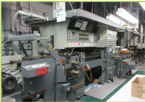
BOBST LEMANIC ROTOGRAVURE W/ IN-LINE PLA 650 ROTOGRAVURE PRINTING PRESS W/ IN-LINE PLATEN DIE CUTTER, CALIPER RANGE .010" TO .040", 12.75" TO 26" MATERIAL RANGE, LINE SPEED 180 METERS/MIN (590 FT/MIN), MAX ROLL OD 72", CORE ID 12", 10-STATIONS, 2-REVERSIBLE STATIONS, ELECTROSTATIC STATIONS; 1,2,3,4,5,6,7,8,9, CYLINDER REPEAT RANGE 17.8" TO 25.6", 144" ELECTRIC OVEN, REGISTER CAP P/P ± 008", P/C AND P/E ± .020", ROTARY P/E ± .020", (REGISTRON S3000) TURRET ROLLSTAND, ROTARY EMBOSsing, BUTT SPLICER, 650 SPARE PARTS, 650 ROLLS, 650 INK POTS & PARTS, Q100M VISION SCANNER. YEAR 1977
