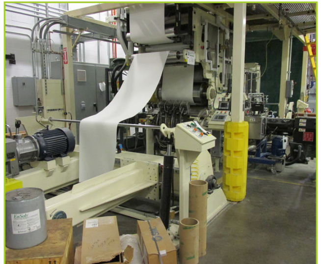
RETROFLEX SLOT DIE COATER ROLL STAND, W/ UNWIND-REWIND CAP., STEEL MAIN FRAME & ROLL FRAMES, SLOT DIE SUPPORT AND POSITION SETTINGS, BACK UP ROLL, ALIGNMENT ROLL, CHILL ROLLS, COATING STATION DRIVE SYSTEM, SMOOTHING ROLL, STATIC BAR, GUIDE ROLLS, STERLING GPAC-30 CHILLING UNIT, 3-STERLING MZB2020-C TEMP CONTROL UNITS, WEB GUIDES, DEGAUSSING BAR, 5-SET FIXED SLOT HOT MELT COATING DIES, 4-POSTION DISPLACEMENT GEAR MELT PUMPS - TYPE 36/36-01, CONTINUOUS SCREEN CHANGER - TYPE K-SWE-121 .YEAR 2011
