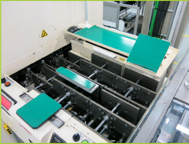
EUNIL ENC-800D INSPECTION CONVEYOR, LENGTH (MM) 1000; MIN WIDTH 30 (MM); MAX WIDTH 205 (MM); DUAL LANE
