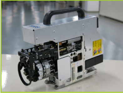
FUJI NXT H12S PLACEMENT HEAD
