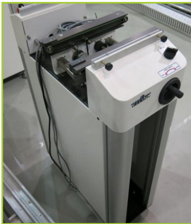
YOUNGJIN FA ACC-30SD BUFFER CONVEYOR LENGTH (MM) 300; MIN WIDTH 30 (MM); MAX WIDTH 250 (MM)
