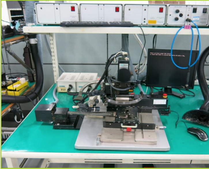
FINETECH PICO FINETECH PICO HIGH DENSITY REWORK STATION
