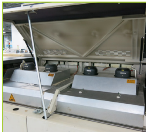
ERSA HOTFLOW 2/14 FLOW DIRECTION: LEFT TO RIGHT; HEATING ZONES: TOP 7/BOTTOM 7; COOLING ZONES: TOP 2/BOTTOM 2; NITROGEN EQUIPPED; EDGE RAIL BOARD TRANSPORT ; CENTER BOARD SUPPORT; AUTO OILER; WATER COOLING; DUAL LANE. S/N: R009A-05C0172. MANUFACTURED IN 2005
