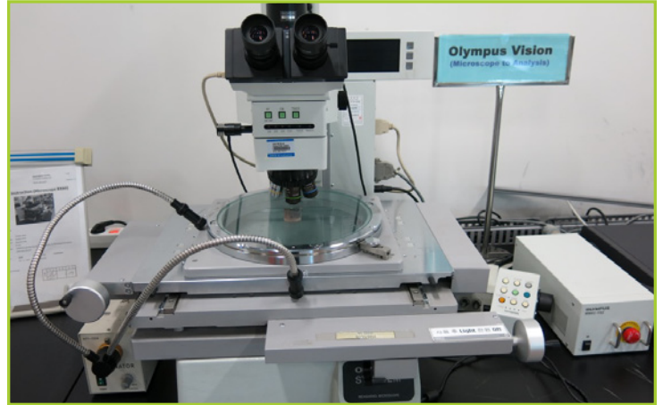
OLYMPUS STM6-LM-F31-2 COMPACT MANUAL 3-AXIS MEASURING MICROSCOPE, 2006
