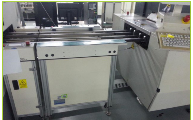
EUNIL EWT-100 INSPECTION CONVEYOR, LENGTH (MM) 1100; MIN WIDTH 30 (MM); MAX WIDTH 205 (MM) ; DUAL LANE
