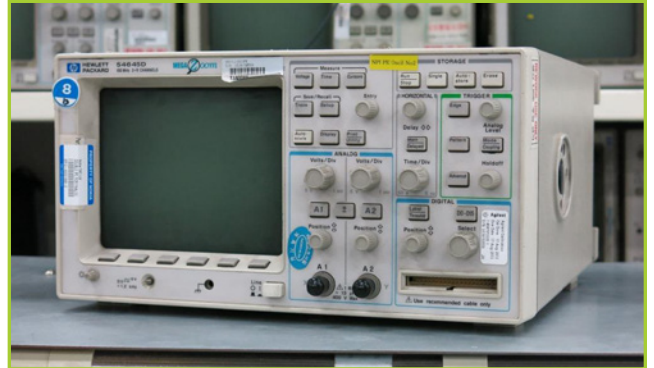
HEWLETT PACKARD 54645D 100-MHZ SCOPE WITH 200 MSAS, 1 MB OF MEMORY PER SCOPE CHANNEL 16 LOGIC TIMING CHANNELS WITH 400 MSAS ON 8 CHANNELS, 200 MSAS ON 16 CHANNELS, 2 MB OF MEMORY PER LOGIC CHANNEL, AGILENT MEGAZOOM TECHNOLOGY ALLOWS DEEP MEMORY CAPTURE
