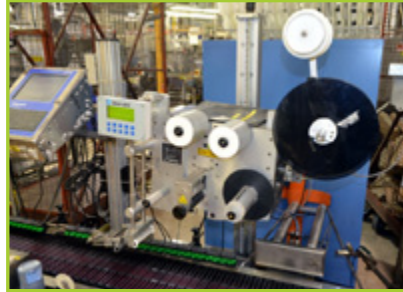
LABEL-AIRE 3115-1500 4/12" LH LABELER
