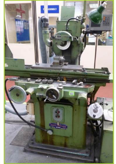
JONES & SHIPMAN 1400 SURFACE GRINDER 24" X 8" CAP, MAG CHUCK, HEIDENHAIN XY DRO
