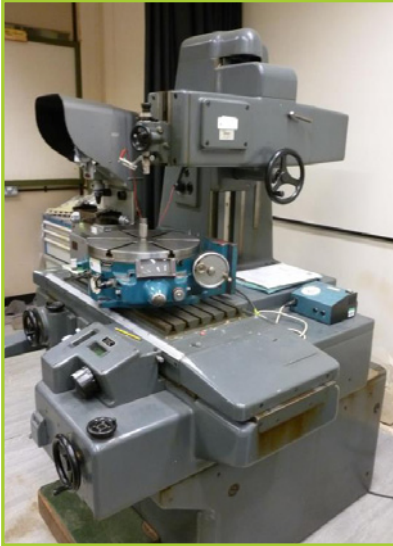
SIP GENEVOISE MU-2M MATERIALS MEASURING SYSTEM VERTICAL JIG BORING & MILLING MACHINE
