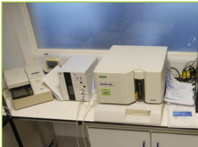
BIO RAD BIO PLEX 200 SUSPENSION ARRAY SYSTEM OPERATING 15-30DEGC, HUMIDITY NONCONDENSING 20-80% WITH BIO PLEX PRO WASH STATION & HTF SYSTEM, 1 X 96 WELL MICROTITRER PLATE CAP, 532NM LASER
