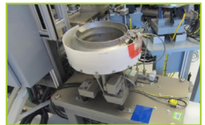
BOWL & TRACK FEEDERS. LOT CONTAINS 8 FEEDERS: ((4) HOMER CITY AUTOMATION EB1 12-A BOWL FEEDERS, (1) WITH HOMER CITY AUTOMATION LD -8 TRACK FEEDER (3) WITH HOMER AUTOMATION LD-4 TRACK FEEDERS), (1) MILLERS FEEDER SOLUTIONS BOWL FEEDER & ((3) PERFORMANCE FEEDERS (1) POSITIVE TERMINAL FEEDER (1) NEGATIVE GROUND FEEDER & (1) TRACK FEEDER).
