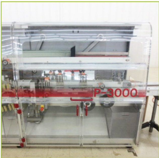
KLOCKNER CP-1200, P-3000 BLISTER MACHINE AND CARTONER PACKAGING LINE . CAPABLE OF THERMOFORMING, COLDFORMING AND CARTONING AT SPEEDS UP TO 400 BLISTER PACKS/MIN AND 300 CARTONS/MIN. WITH HASKRIS CHILLER, GREYDON MDL. 01SBM053 PRINTER S/N 325BPP. WITH MANUALS. WITH 3 CRATES OF ADDITIONAL RAILS.
