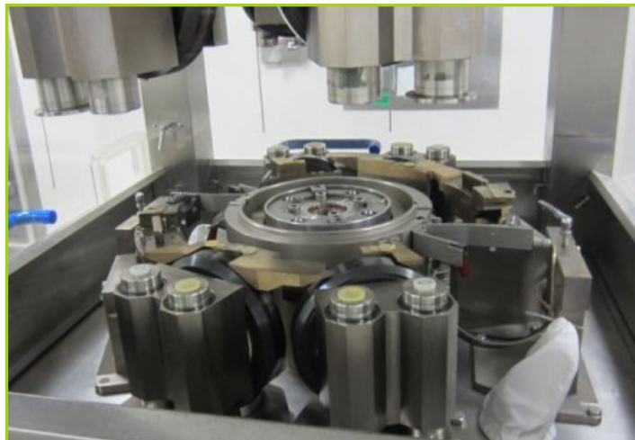
FETTE P3090 IC TABLET PRESS. 49 STATION ROTARY TABLET PRESS , TURRET IN STORAGE STAND WITH ELECTRICAL PANEL MAIN CONTROL PANEL. ALL CABLES, RATED UP TO 700,000 TABLETS PER HR, METRO RACK WITH ASSORTED PARTS, YR 1999. SN# 29 264
