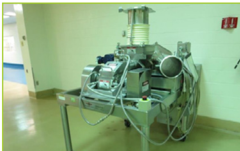
FITZPATRICK COMPANY DKAS06 FITZMILL COMMINUTOR , 10" INLET, 8" DISCHARGE, WITH 8" X 55" SS CHUTE. EXPLOSION PROOF ELECTRICAL BOX, SET UP TO USE ON DISCHARGE BIN
