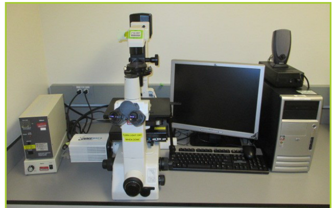
NIKON ECLIPSE TE300 INVERTED RESEARCH MICROSCOPE. FEATURES: 6-POSITION NOSEPIECE WITH THE FOLLOWING OBJECTIVES: (1) PLAN FLUOR ELWD 40X/0.60 PH2 DM \sim /0-2 WD 0.37-0.27, (1) PLAN FLUOR 20X/0.45 PH1 DM \sim /0-2 WD 7.4, (1) PLAN FLUOR 10X/0.30 PH1 DLL \sim /0.17 WD 16.0, (1) PLAN FLUOR 4X/0.13 \sim /- WD 17.1; (2) CFI 10X/22 EYEPIECES; CONDENSER TURRET, UV FLUORESCENCE CASSETTE, 12V 100W LAMPS, MULTIPLE LIGHT FILTERS; XY EXTENDED KNOB STAGE, Z-AXIS CONTROL. INCLUDES: PHOTOMETRICS COOLSNAP FX HIGH-RESOLUTION SCIENTIFIC CAMERA; HIGH PRESSURE MERCURY LAMP POWER SUPPLY, HALOGEN LAMP POWER SUPPLY; AND MORE
