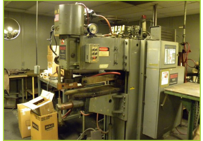
SCIAKY PRESS TYPE 3 PHASE SPOT WELDER MODEL #11297. TYPE: PMCO 1STM75365, 440VAC, 60HZ, SEC. AMPS 60K -8'HX9' LX3.5' W 3.5', DEEP THROAT
