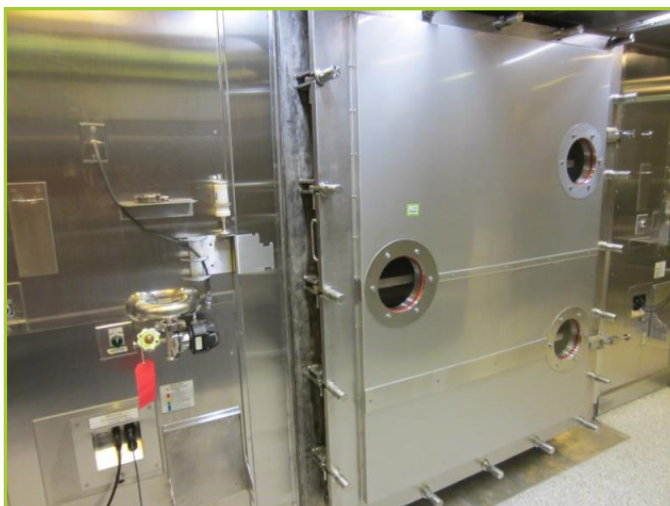
STOKES 264 SQ FT. FREEZE DRYER. REBUILT IN 2008. 2 SKIDS, CONDENSER & REFRIGERATION. UP GRADED CONTROLS WITH OLD CONTROLS FOR BACKUP
