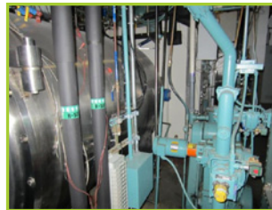
STOKES 264 SQ. FT. FREEZE DRYER. CHAMBER MAWP 18PSI @ 260°F, MDMT -20°F @ 18PSI 2 SKIDS, REBUILT IN 2008, CONDENSER YR 2003 & REFRIGERATION (2) COPELAND 6TM1-2000-TSK-800 COMPRESSORS. UP GRADED CONTROLS WITH OLD CONTROLS FOR BACKUP.
