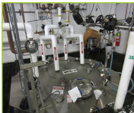
16,500 LITER STAINLESS STEEL TANK. VESSEL VOLUME 5000GAL, VESSEL M.A.W.R.50-15 PSI @350°F, NATIONAL BOARD # 4626. 8'6" DIA X 11' .500THK 316L STEEL YR 2000 NON JACKETED.YEAR: 2000
