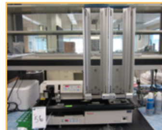
CARTESIAN TECHNOLOGIES HUMMINGBIRD 384 XL
