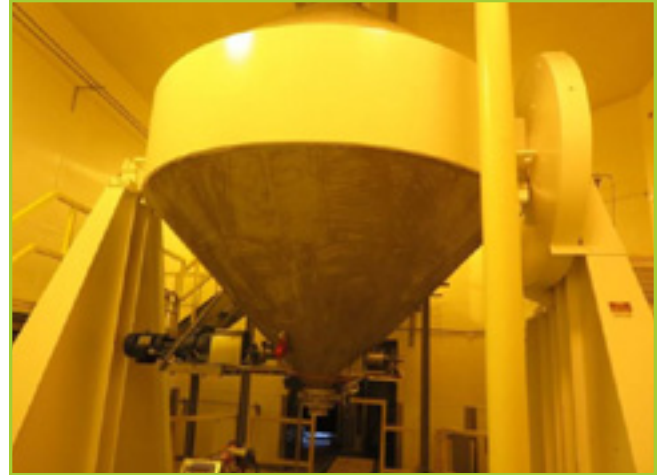
THOROBLENDER. 10' DIA. WELDED CONSTRUCTION, BUILT IN DELUMPER, MATERIAL: ALL PARTS CONTACTING PRODUCT 316 L.S.S., INTERIOR FINISH: P2 SEMI POLISH FINISH, TOTAL VOLUME 454 CU. FT., WORKING VOLUME 320 CU. FT. @80LBS CU.FT. DENSITY. TOTAL EST. WT. 18,950LBS, VESSEL DESIGNED FOR 2" HG INTERNAL VACUUM, BLENDER SPEED 12.9 R.P.M. WITH 28" W X APPROX 25FT OF CONVEYOR & STAIRS & CAT WALK SURROUNDING BLENDER.
