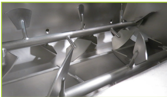
2006 AMFEC 2,000 LB CAPACITY S/S DUAL PADDLE BLENDER, MODEL: 510, S/N: 070406, WITH CO2 INJECTION MOUNTED ON LOAD CELLS, WITH PLATFORM, STARTERS, AND CONTROLS
