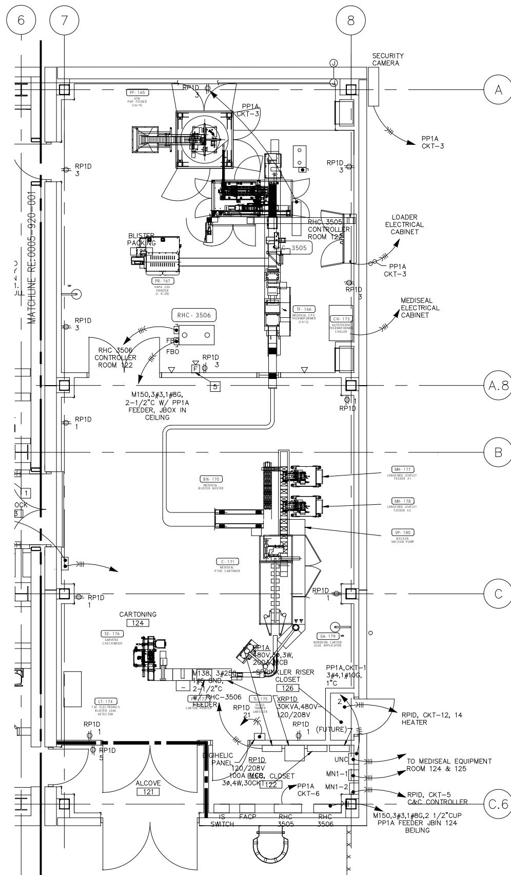
1 ANNEX FIRST FLOOR POWER PLAN SCALE: 1/4"=1'-0"
